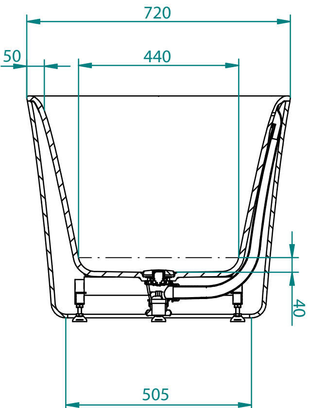
SECTION B-B
